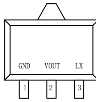
SOT89-3L (Top View)
